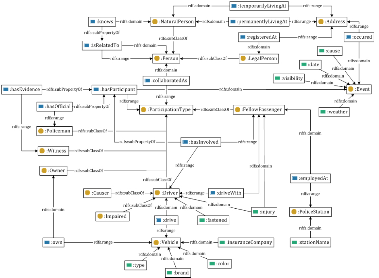
Fig. 2. Ontology representing various classes, relations and attributes related to traffic accidents and automobile insurance domain. Classes are colored with orange, relations with blue and attributes with green. Key concepts of the ontology are Event , Person , Driver , Witness , Owner and Vehicle .
