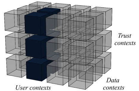
Fig. 4. Characterization of merging and matching execution defining one context in user dimension, two contexts in data dimension and all contexts in trust dimension.
