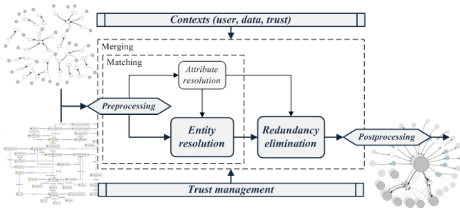
Fig. 6. General framework for matching and merging data from heterogeneous sources.
